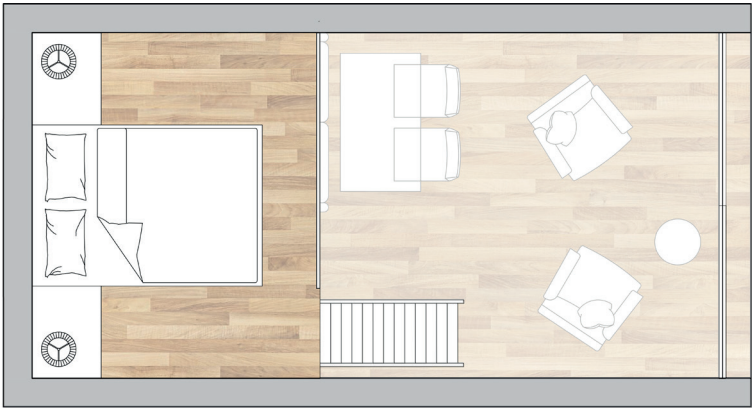
Floor Plan - Mezzanine
