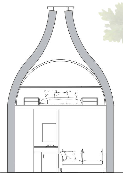
Section
